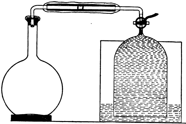
FIG. 153.—Gas-collecting apparatus.
